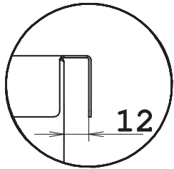
DETAIL A 1:2
